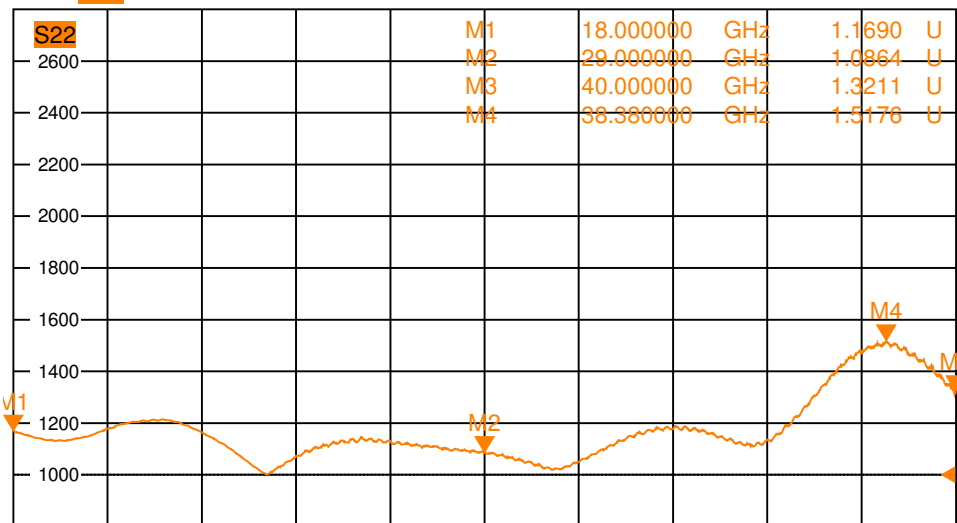
Ch1 Base Freq Start 18 GHz Base Pwr 0 dBm Stop 40 GHz
